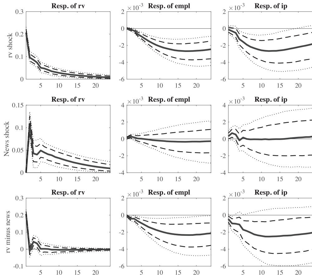
FIGURE 2 IRFs from benchmark VAR.
