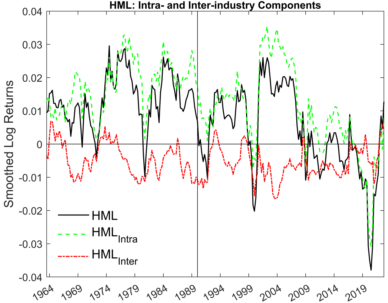
Figure 2: We plot the results from the Table 2 decomposition of HML into its intra- and inter-industry components for the Compustat period from 1963Q3-2022Q4. The solid black line shows the smoothed log return to Fama and French's (1993) HML; the dashed green line shows the smoothed log return to the intra-industry component of HML; and the dashed-dotted red line shows the smoothed log return to the inter-industry component. The series are smoothed with a trailing exponentially weighted moving average in which the decay parameter is set to 0.08 per quarter, and the smoothed series is generated, for example, as MA_t(\text{HML}) = 0.08\text{HML}_t + (1-0.08)MA_{t-1}(\text{HML}) . This decay parameter implies a half-life of two years. The vertical line indicates the start of the subperiod 1990Q2-2022Q4.
