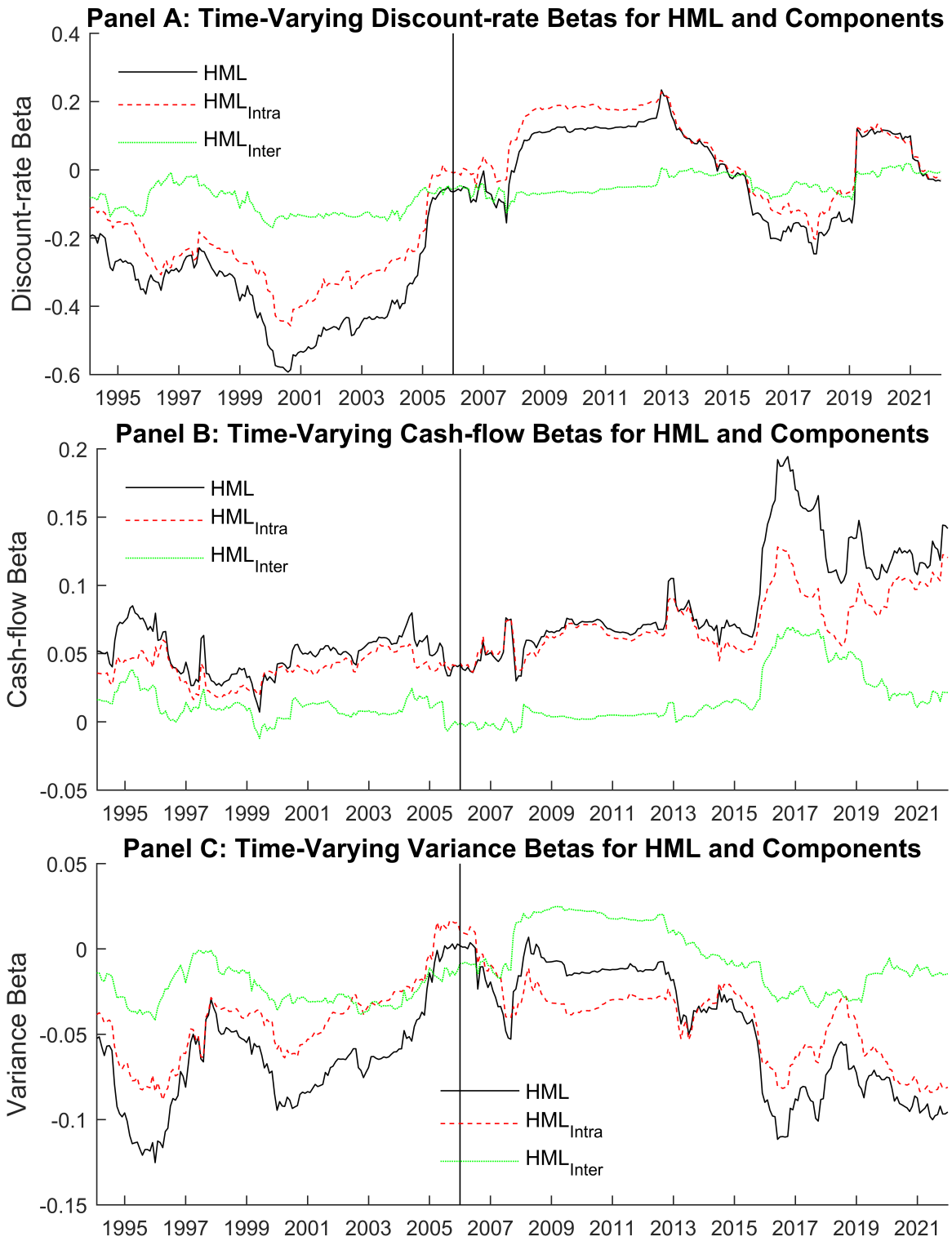
Figure 10: We plot discount-rate ( \hat{\beta}_{DR} ) (Panel A), cash-flow ( \hat{\beta}_{CF} ) (Panel B), and variance ( \hat{\beta}_V ) betas (Panel C) for HML (solid black line), HML_{Intra} (dashed red line), and HML_{Inter} (dotted green line) that we estimate using monthly observations within five-year rolling windows. The vertical line indicates the end of 2006Q4, since then, the cumulative return to HML has been -50%.
