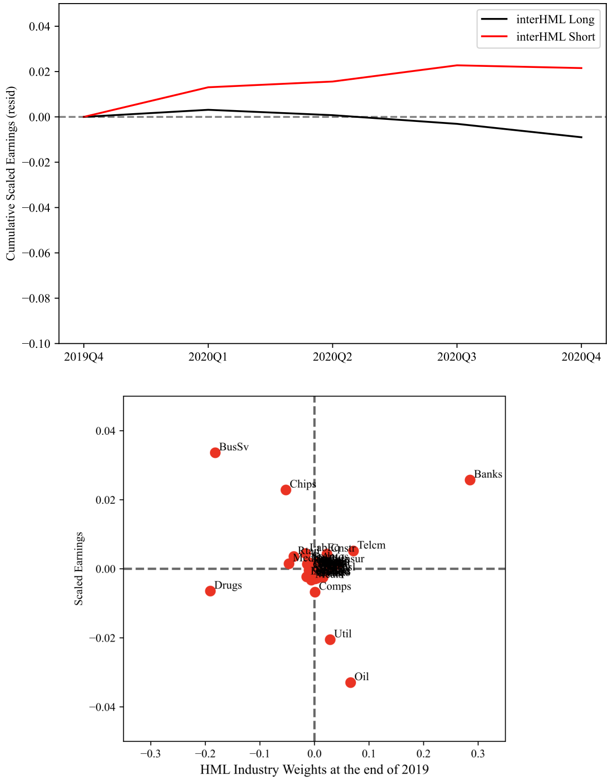
Figure 9: The top panel shows the cumulative earnings during 2020 (scaled by total book equity in 2019q4, ScaledCumulEarn_{t,t+h}^p ) for the long side (black line) and short side (red line) of the inter-industry HML portfolio. Both are residualized to the market earnings. The bottom panel reports HML's weights in each industry at the end of 2019 on the X axis and that industry's contribution to HML's cumulative earnings in 2020 on the Y axis, again residualized to the aggregate earnings.
