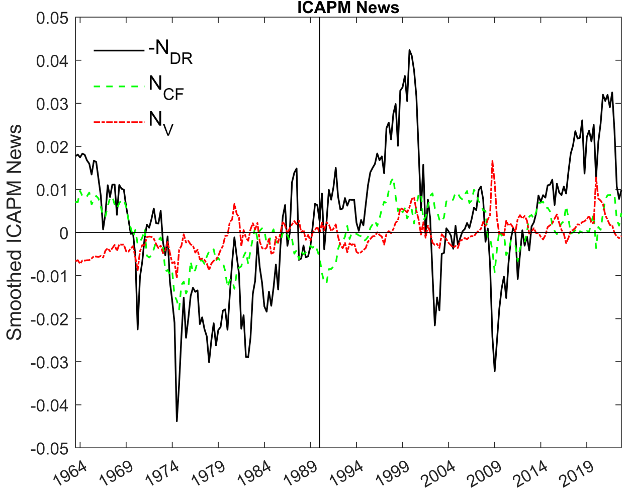
Figure 3: We plot smoothed ICAPM News for the Compustat subsample from 1963Q3-2022Q4 as generated by the VAR in Appendix Table 1. The solid black line shows the negative of smoothed aggregate discount-rate news; the dashed green line shows smoothed aggregate cash-flow news; and the dashed-dotted red line shows smoothed aggregate variance news. The series are smoothed with a trailing exponentially weighted moving average in which the decay parameter is set to 0.08 per quarter, and the smoothed series is generated, for example, as MA_t(N^{CF}) = 0.08N_t^{CF} + (1-0.08)MA_{t-1}(N^{CF}) . This decay parameter implies a half-life of two years. The vertical line indicates the start of the subperiod 1990Q2-2022Q4.
