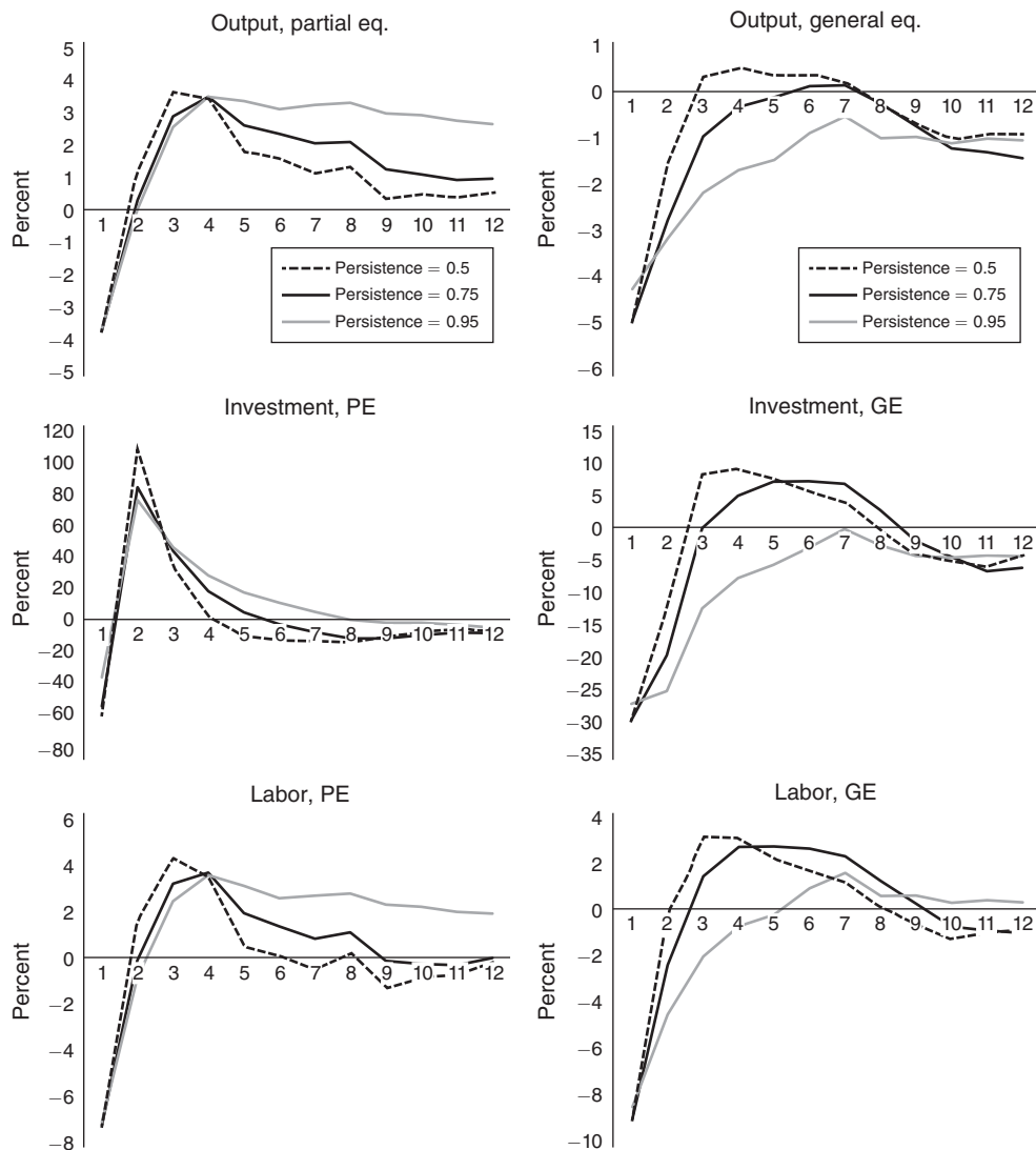
FIGURE A1. IRFs IN THE RUBC MODEL
